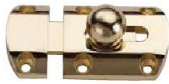
Number C726 Length 63mm Width 34mm
