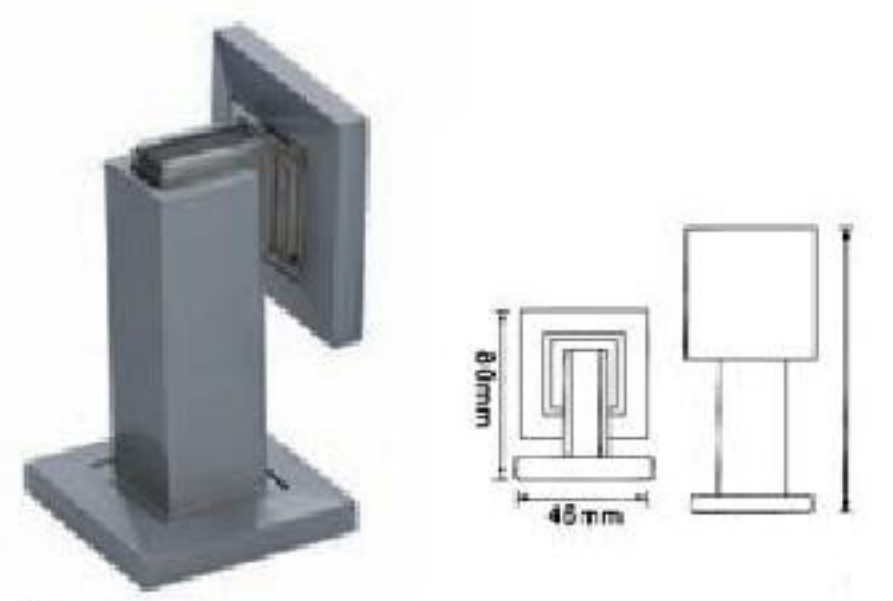
■ MODEL: G-6188 MATERIAL: ZINC ALLOY
