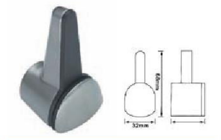
■ MODEL: G-6187 MATERIAL: ZINC ALLOY
