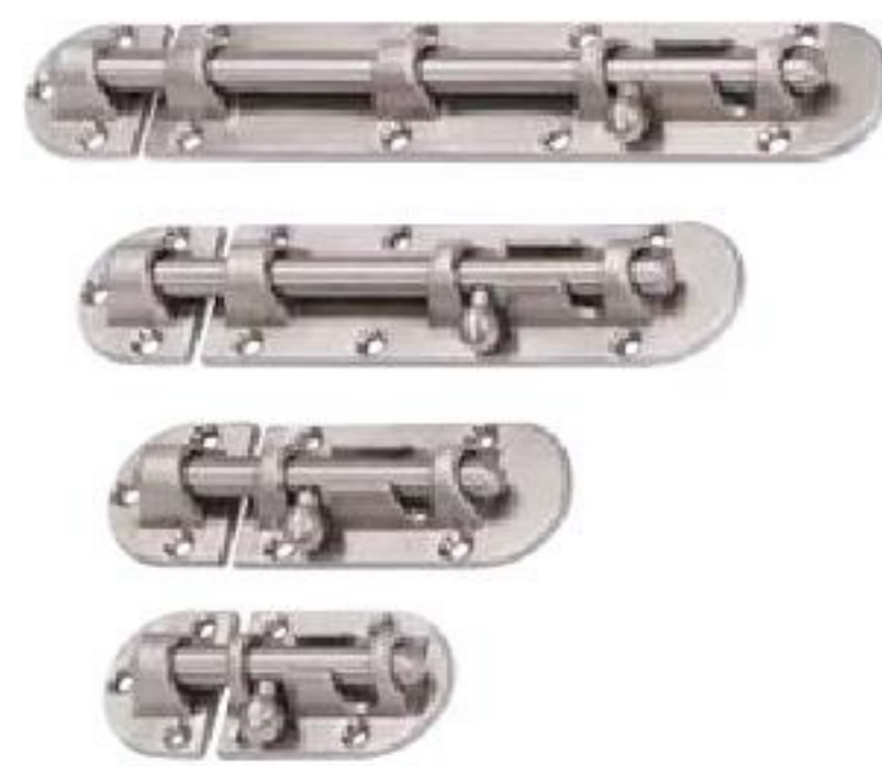
Number C647 Length 8" 6" 4" 3" Width 34mm 34mm 34mm 34mm
