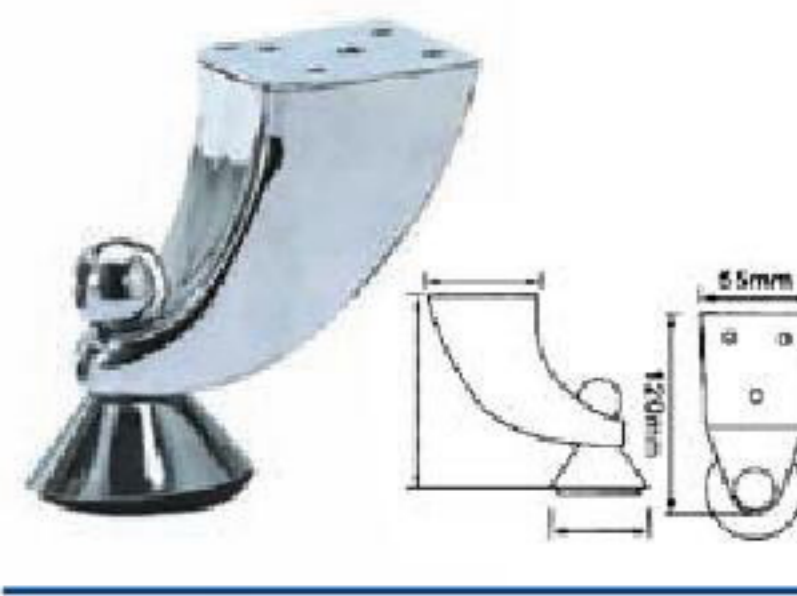
■ MODEL: G-6138 MATERIAL: ZINC ALLOY
