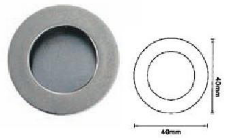
■ MODEL: G-6110 MATERIAL: ZINC ALLOY
