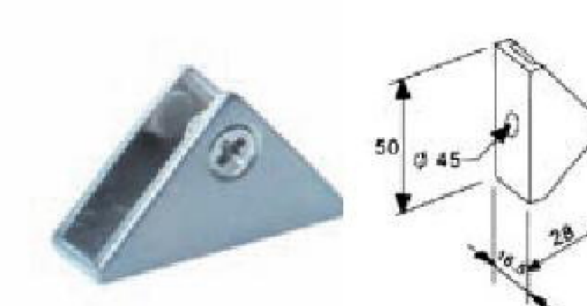
■ MODEL: G-6194 MATERIAL: ZINC ALLOY
