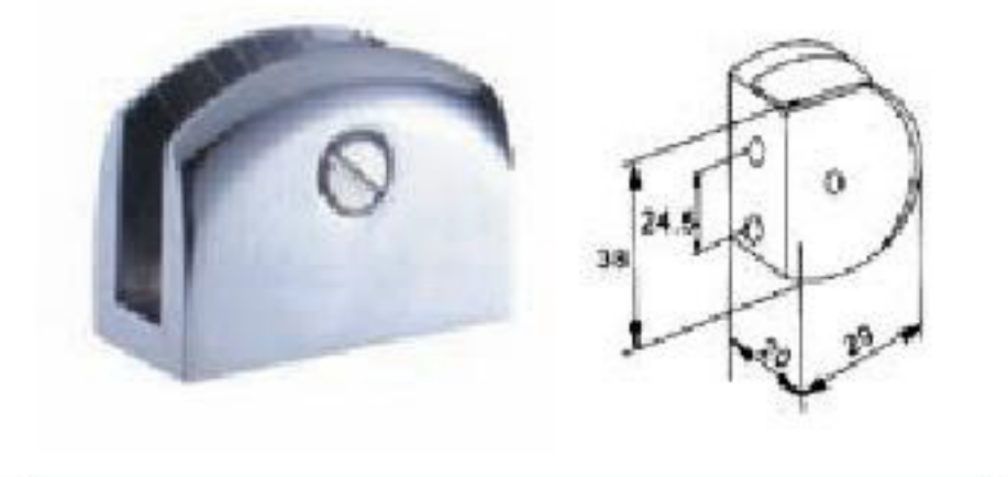
■ MODEL: G-6191 MATERIAL: ZINC ALLOY
