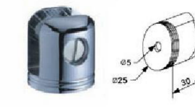
■ MODEL: G-6197 MATERIAL: ZINC ALLOY
