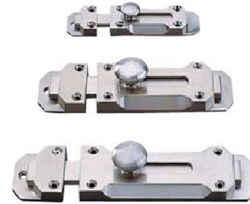
Number C966 Length 63mm Width 34mm Height 24mm
