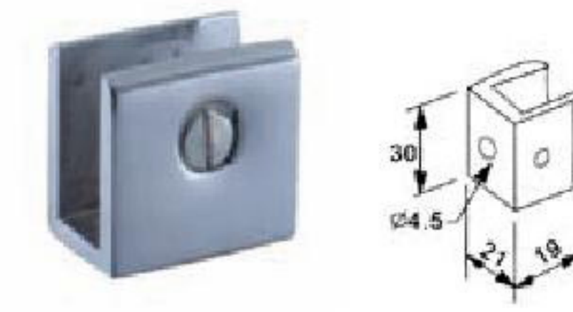
■ MODEL: G-6192 MATERIAL: ZINC ALLOY
